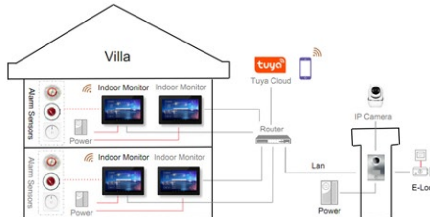
TC-5000MH-20H + TC-3000DA-X2
